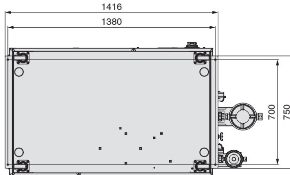
Anchor bolt mounting position (View A)
