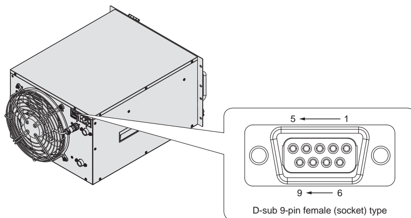
Communication connector
